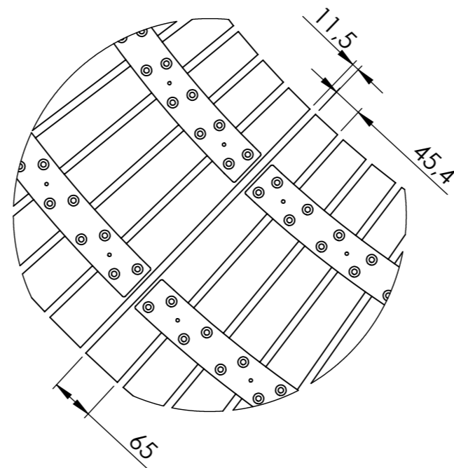
DETAIL A
